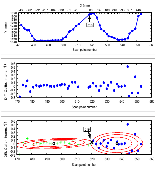
Fig. 4: Segment separation: (a) scan data in Cartesian coordinates, (b) \mathcal{D} data, (c) EM for segment separation, “○” estimated mean of each Gaussian, “X” breakpoint.
